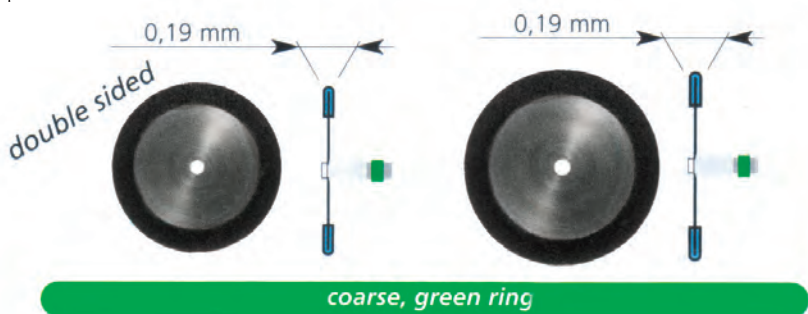
FLEXIFLEX® 5' - 10000 rpm (low)
