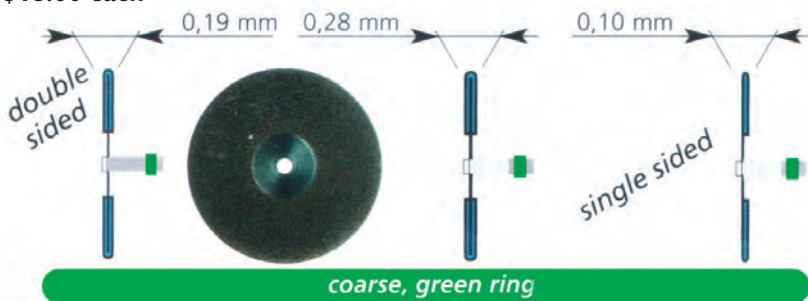
TOTO-FLEX 5' - 10000 rpm (low)
